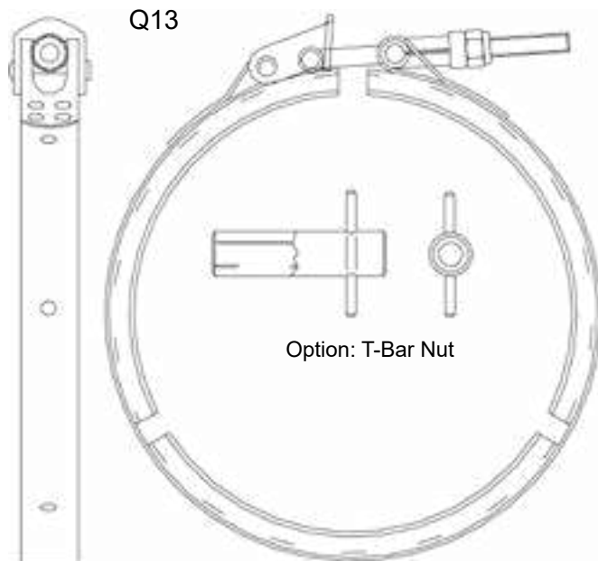
T-Bolt, Quick Coupler, three Segments
