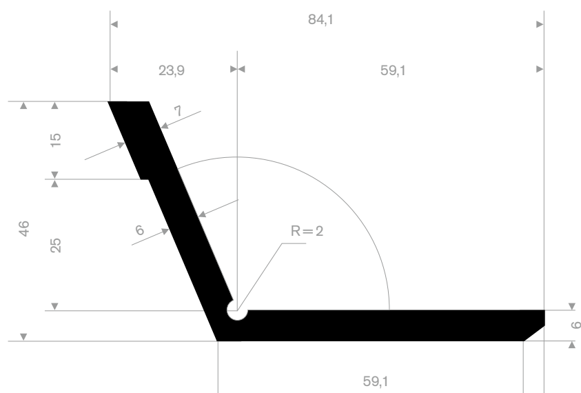
EPDM 70° Shore black roll length 4 meter
