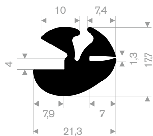
EPDM 70° Shore black roll length 50 meter
