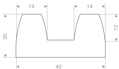
TPE 60° Shore white roll length 25 meter
