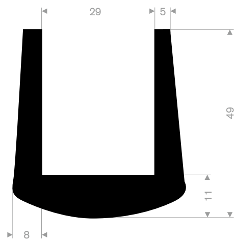
EPDM 70° Shore black roll length 25 meter
