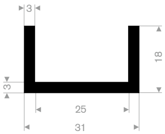
EPDM 70° Shore black roll length 25 meter
