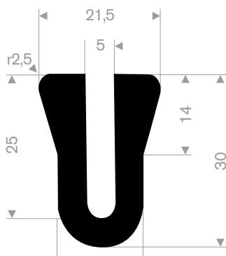
EPDM 70° Shore black roll length 50 meter
