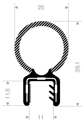
pvc + Sponge rubber clamping range 9-10,5 mm roll length 50 meter
