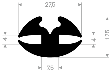
EPDM 70° Shore black roll length 50 meter
