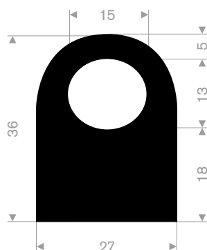
EPDM 40° Shore black roll length 20 meter
