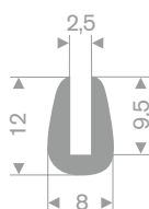
TPE 70° Shore grey roll length 100 meter
