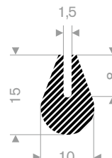
EPDM 15° Shore black roll length 100 meter
