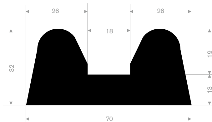
EPDM 65° Shore black roll length 15 meter
