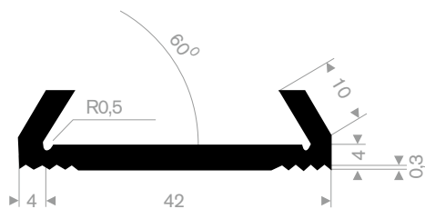
EPDM 70° Shore black roll length 50 meter
