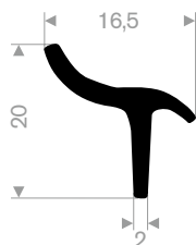
EPDM 70° Shore black roll length 30 meter
