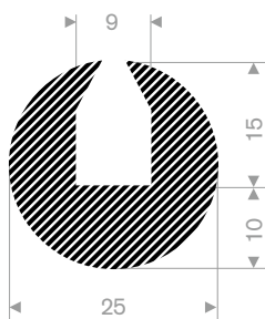
EPDM 15° Shore black roll length 30 meter
