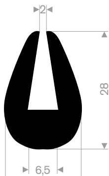
EPDM 70° Shore black roll length 50 meter
