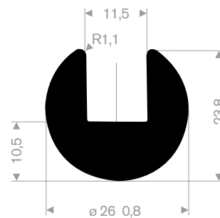
EPDM 70° Shore black roll length 50 meter
