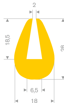
TPE 70° Shore yellow roll length 50 meter
