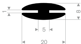
EPDM 70° Shore black roll length 100 meter
