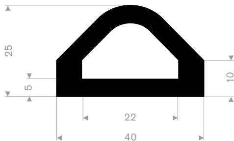
EPDM 70° Shore black roll length 5 meter
