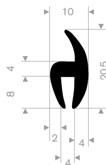
EPDM 70° Shore black roll length 50 meter
