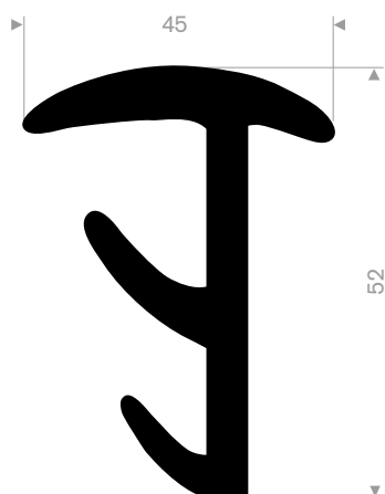
EPDM 70° Shore black roll length 25 meter
