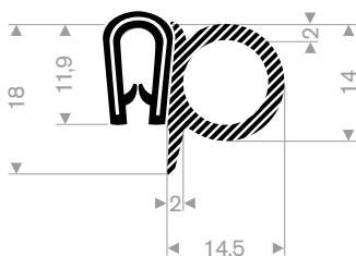
pvc + Sponge rubber clamping range 1,5-3 mm roll length 25 meter
