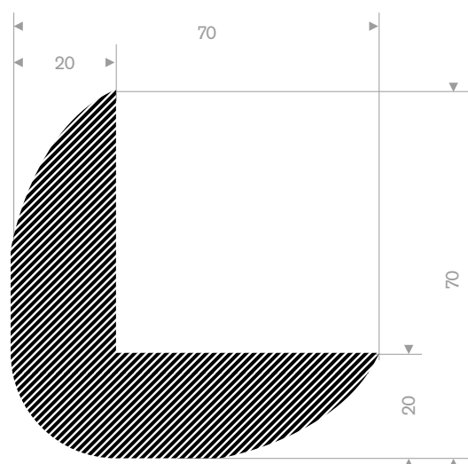
EPDM 15° Shore black roll length 10 meter
