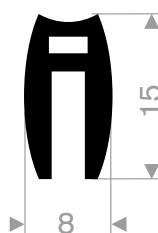
EPDM 65° Shore black roll length 25 meter
