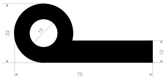
EPDM 70° Shore black roll length 20 meter
