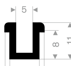
EPDM 70° Shore black roll length 30 meter
