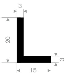
EPDM 70° Shore black roll length 50 meter
