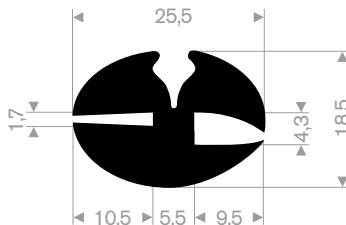
EPDM 70° Shore black roll length 50 meter
