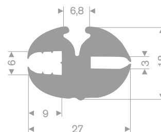
TPE 70° Shore grey roll length 30 meter
