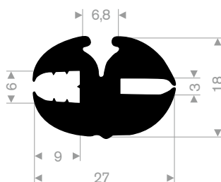
EPDM 70° Shore black roll length 30 meter
