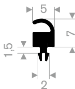
EPDM 70° Shore black roll length 100 meter
