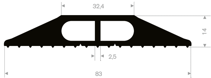
EPDM 70° Shore black roll length 9 meter
