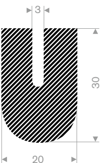
EPDM 15° Shore black roll length 25 meter
