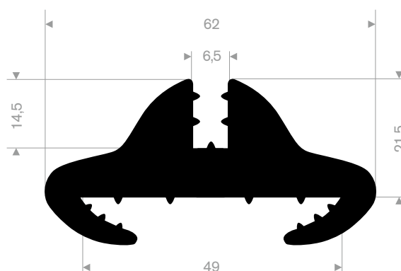
EPDM 70° Shore black roll length 25 meter
