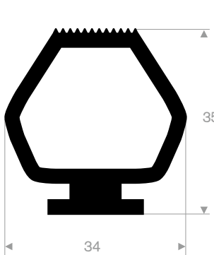
EPDM 70° Shore black roll length 25 meter
