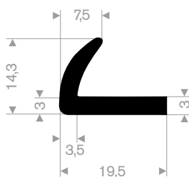
EPDM 70° Shore black roll length 50 meter
