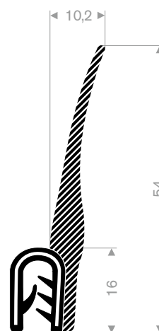
pvc + Sponge rubber clamping range 1,5-5 mm roll length 25 meter
