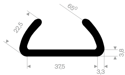
EPDM 70° Shore black roll length 50 meter
