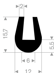
EPDM 70° Shore black roll length 50 meter
