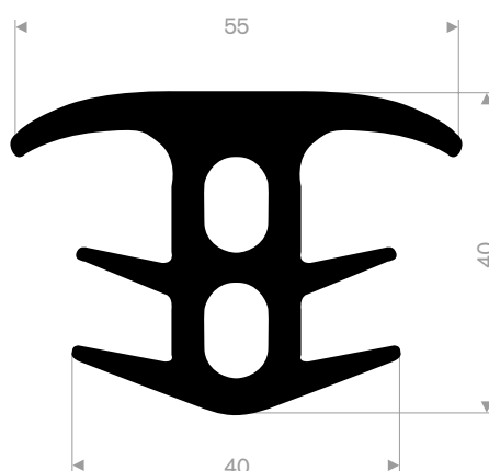
EPDM 70° Shore black roll length 15 meter
