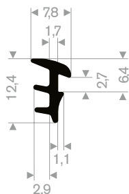
EPDM 65° Shore black roll length 200 meter
