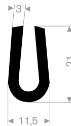
EPDM 70° Shore black roll length 50 meter
