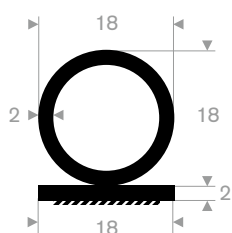
EPDM 90° Shore with adhesive roll length 25 meter
