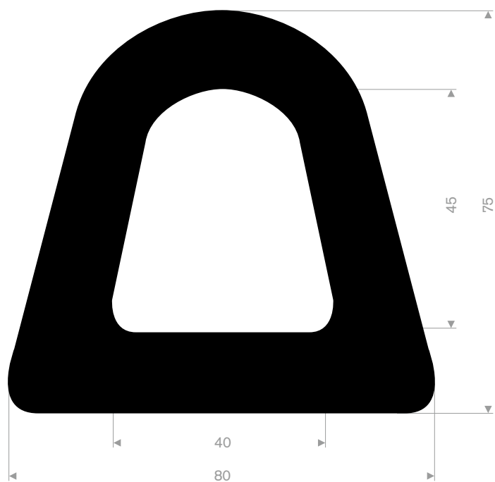
EPDM 70° Shore black roll length 12,50 meter
