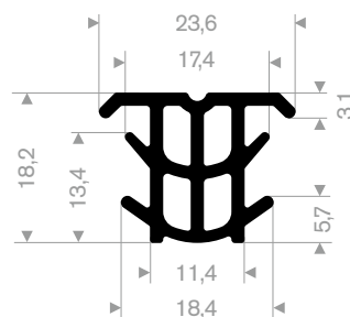
EPDM 70° Shore black roll length 75 meter
