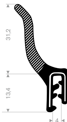
pvc + Sponge rubber clamping range 1,5-4 mm roll length 30 meter
