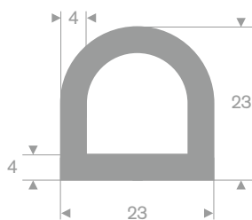
TPE 60° Shore grey roll length 25 meter
