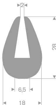
TPE 70° Shore grey roll length 50 meter
