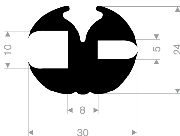
EPDM 70° Shore black roll length 50 meter
