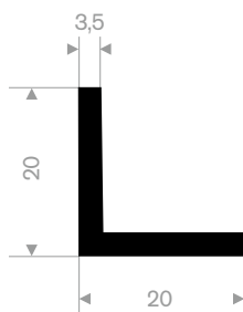
EPDM 70° Shore black roll length 50 meter
