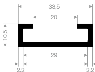
EPDM 70° Shore black roll length 50 meter
