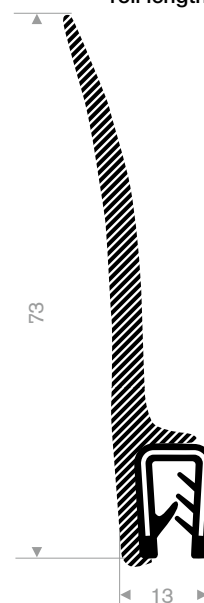
pvc + Sponge rubber clamping range 1-2 mm roll length 25 meter
