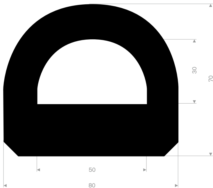
EPDM 70° Shore black roll length 12,50 meter
