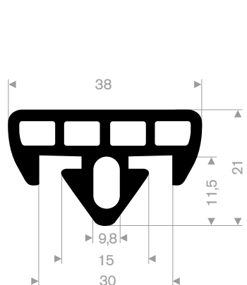
EPDM 70° Shore black roll length 25 meter
