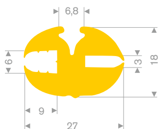
TPE 70° Shore yellow roll length 30 meter
