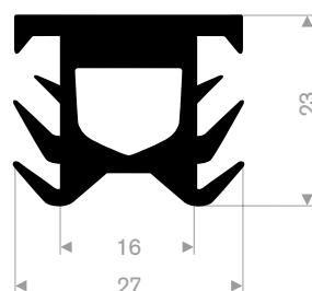
EPDM 70° Shore black roll length 25 meter
