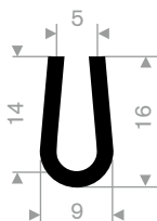
EPDM 70° Shore black roll length 100 meter
