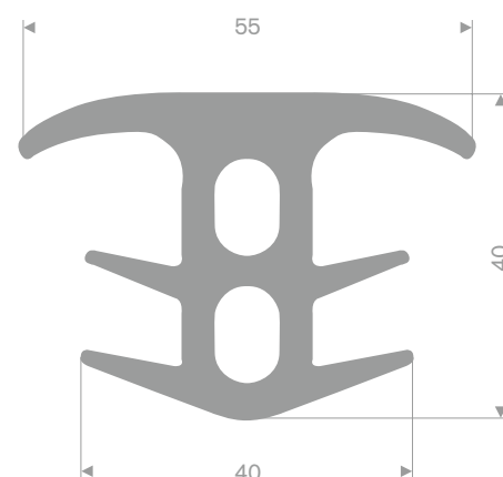
EPDM 70° Shore grey roll length 15 meter
