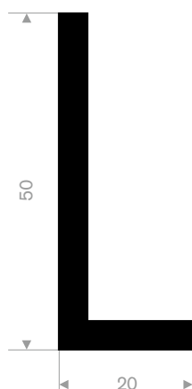
EPDM 70° Shore black roll length 25 meter
