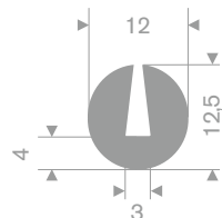
TPE 70° Shore grey roll length 50 meter
