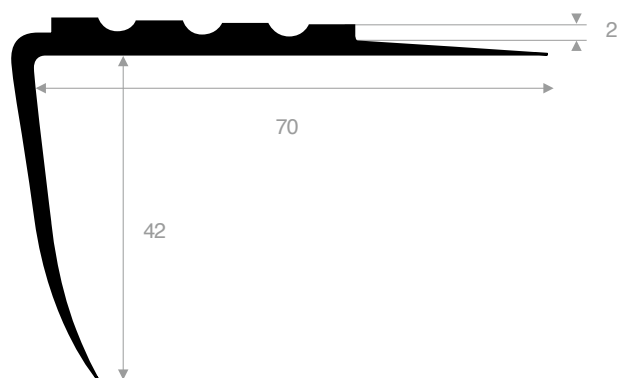
PVC 70° Shore black Length 1,50
