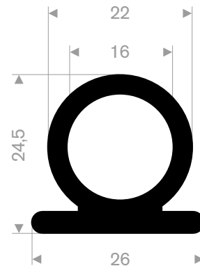
EPDM 70° Shore black roll length 25 meter
