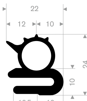
NBR 65° Shore black roll length 25 meter
