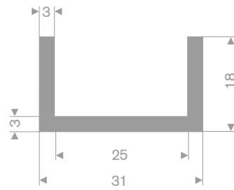
TPE 70° Shore grey roll length 25 meter
