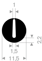
EPDM 70° Shore black roll length 100 meter
