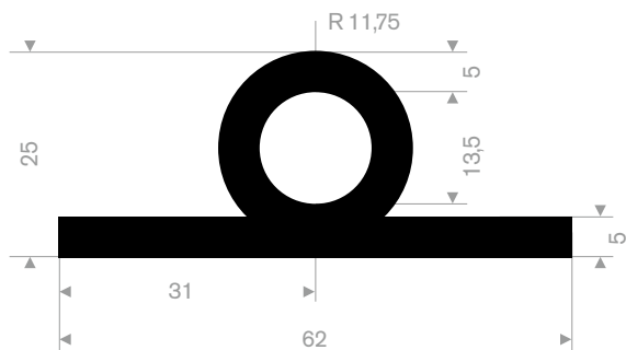
TPE 70° Shore black roll length 25 meter
