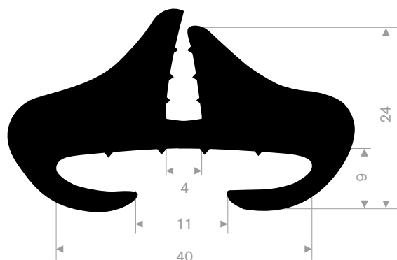
EPDM 70° Shore roll length 30 meter
