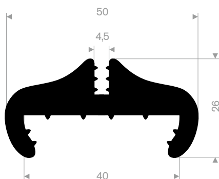
EPDM 70° Shore black roll length 25 meter
