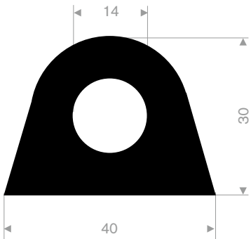
EPDM 65° Shore black roll length 20 meter
