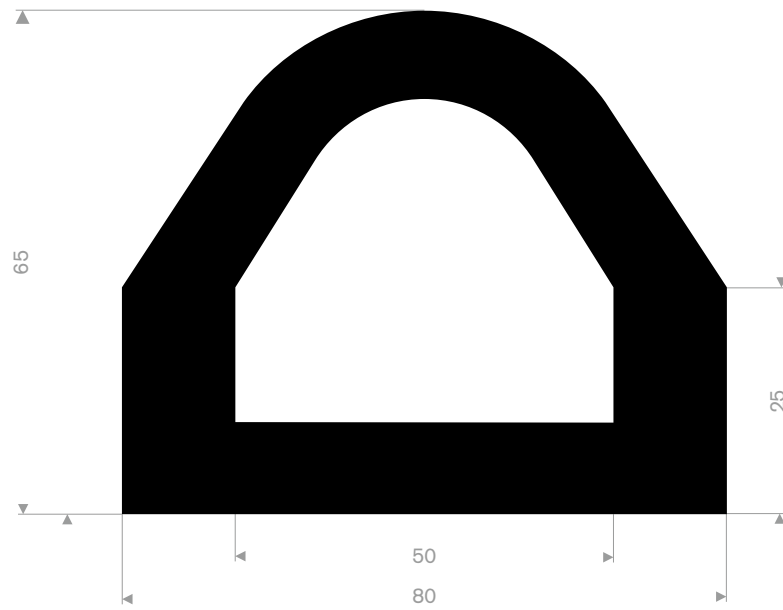
EPDM 70° Shore black roll length 5 meter
