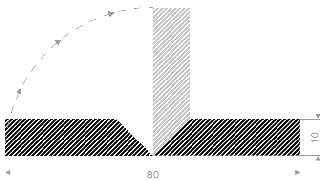
EPDM 15° Shore black length 2 meter
