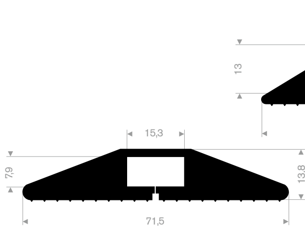
PVC 92° Shore black/yellow roll length 9 meter
