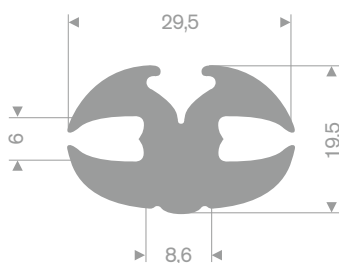
EPDM 70° Shore grey roll length 25 meter
