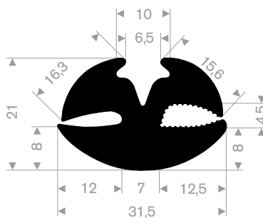
EPDM 70° Shore black roll length 25 meter
