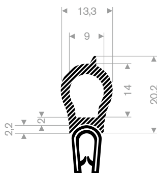
pvc + Sponge rubber clamping range 1-3 mm roll length 50 meter
