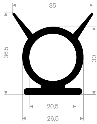
EPDM 70° Shore black roll length 10 meter
