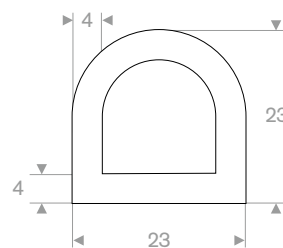
TPE 60° Shore white roll length 25 meter
