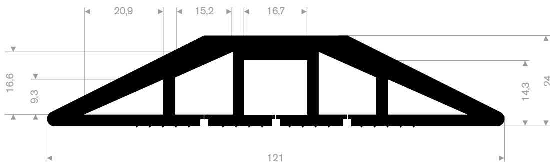
PVC 92° Shore black/yellow roll length 9 meter
