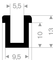
EPDM 70° Shore black roll length 50 meter
