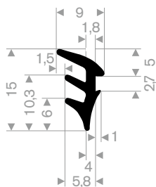
EPDM 65° Shore black roll length 200 meter
