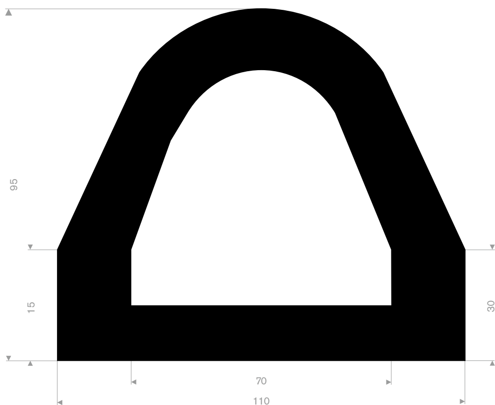
EPDM 70° Shore black roll length 5 meter
