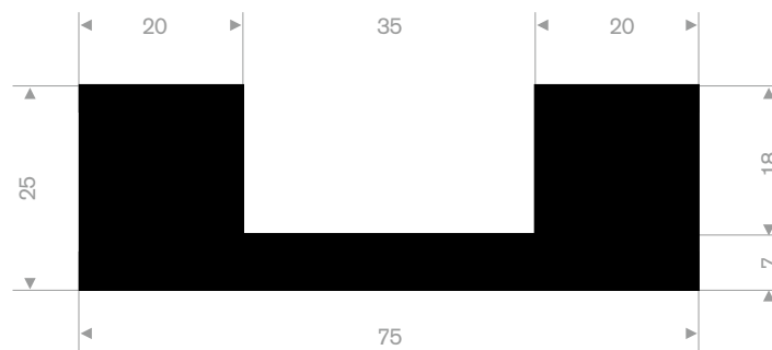
EPDM 70° Shore black roll length 20 meter
