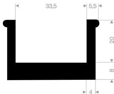
EPDM 70° Shore black roll length 25 meter
