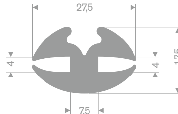
TPE 70° Shore black roll length 30 meter
