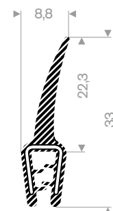
pvc + Sponge rubber clamping range 1-2,5 mm roll length 50 meter
