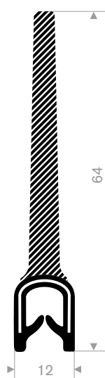
pvc + Solid rubber clamping range 1,5-4 mm roll length 40 meter
