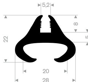
EPDM 70° Shore black roll length 20 meter
