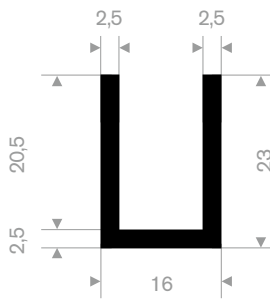
EPDM 70° Shore black roll length 50 meter
