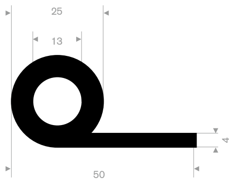
EPDM 70° Shore black roll length 25 meter
