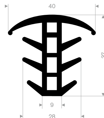
EPDM 70° Shore black roll length 25 meter
