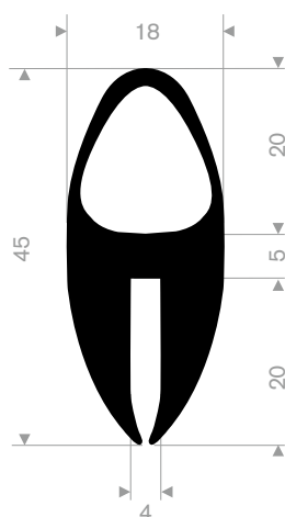
EPDM 65° Shore black roll length 50 meter
